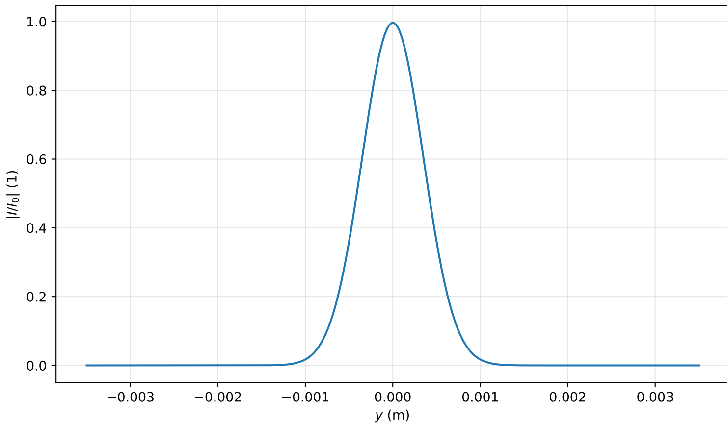
Intensity profile I(x=0, y, z=0.159)/I_0 , \text{Pin}=0.1\text{Pcr} , artificial time
